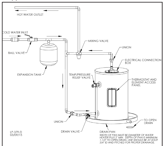
Figure 4 - Piping Detail for o10, o15, and o20 Models - NOTE: Drawing is meant only to demonstrate system piping concept. The installer is responsible for equipment and detailing required by local codes.
