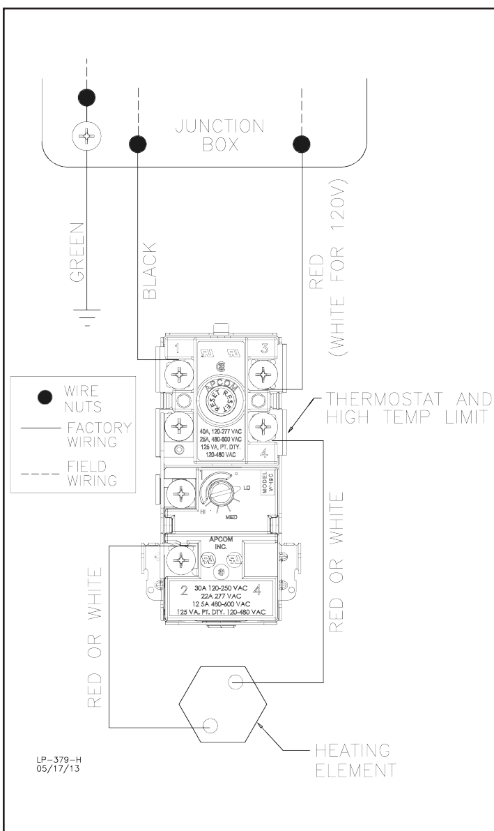
Figure 9 - Single Element Model Wiring Detail (010, 015, and 020 Models ONLY)
