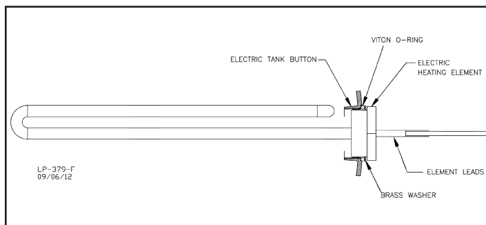
Figure 3 - Heating Element Detail
