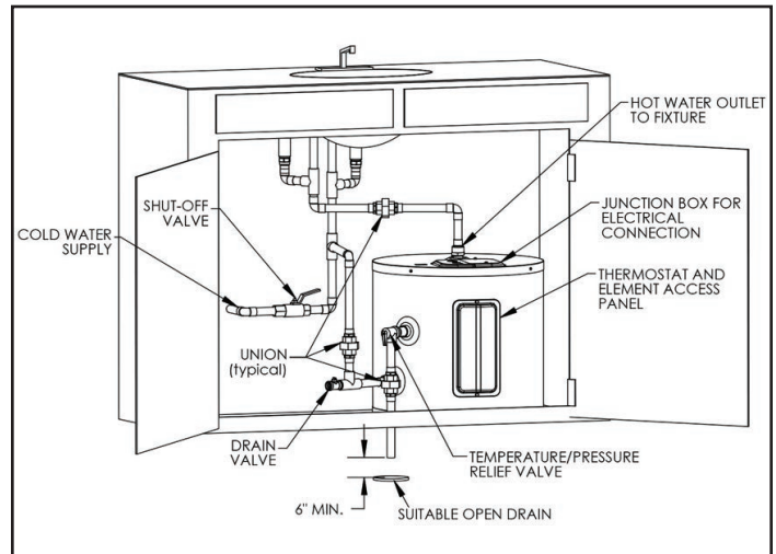
Figure 6 - Point of Use Installation - 010, 015, 020 Models - NOTE: Drawing is meant only to demonstrate system piping concept.
