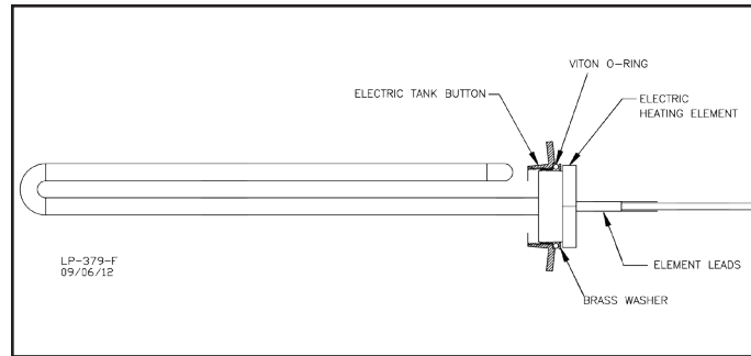
Figure 12 - Heating Element Detail
