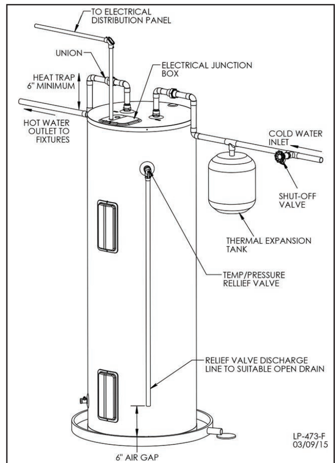
Figure 8 - 80, 100, and 115 Gallon Piping Detail - NOTE: Drawing is meant to demonstrate system piping concept. Heat traps are optional.
