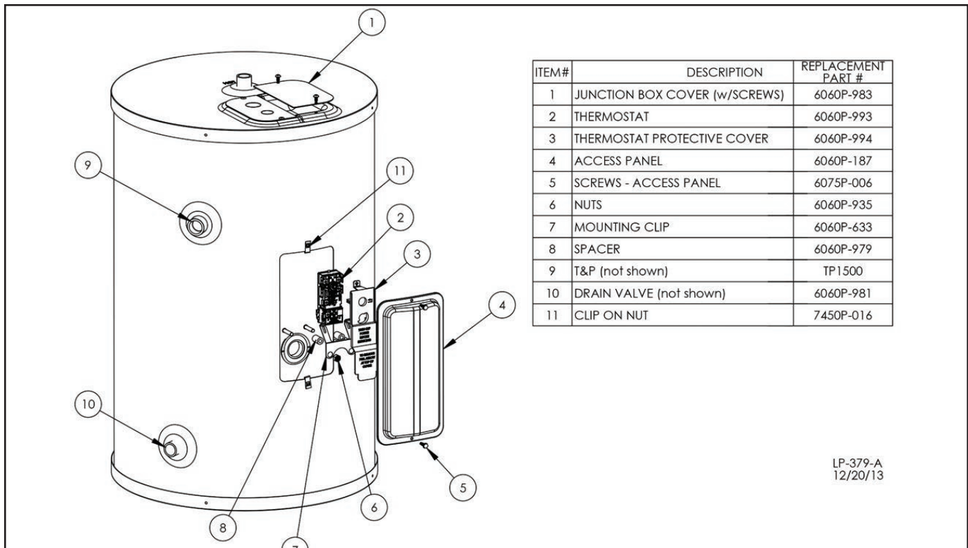
Figure 13 - Replacement Parts - 010, 015, and 020 Models
