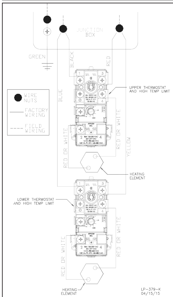
Figure 10 - Dual Element Model Wiring Detail, Simultaneous Operation (030, 040, 050, 080, 100, and 115 Models ONLY)
