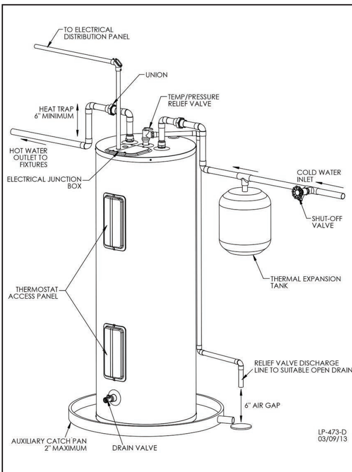
Figure 7 - 30, 40, and 50 Gallon Piping Detail - NOTE: Drawing is meant to demonstrate system piping concept. Heat traps are optional.
