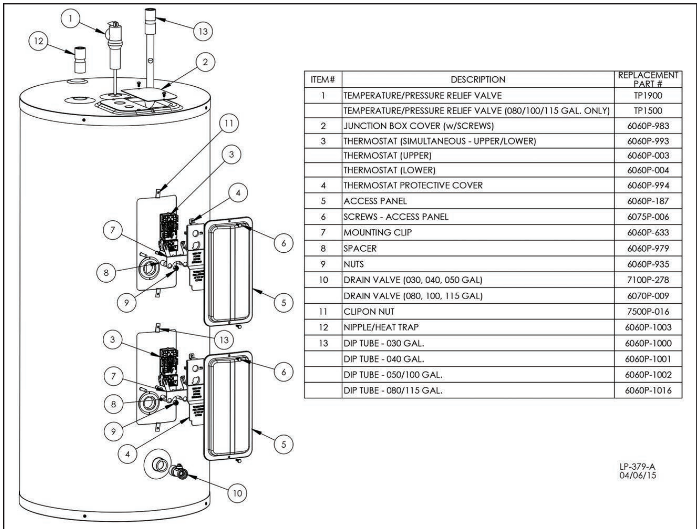
Figure 14 - Replacement Parts - 030, 040, 050, 080, 100, and 115 Models - NOTE: T&P Valve Located on Side of 080, 100, and 115 Models
