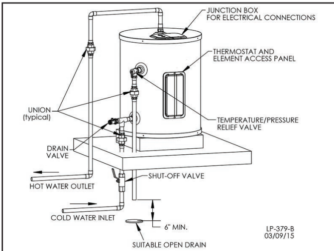
Figure 5 - Mobile Home Installation - 010, 015, 020 Models - NOTE: Drawing is meant only to demonstrate system piping concept.
