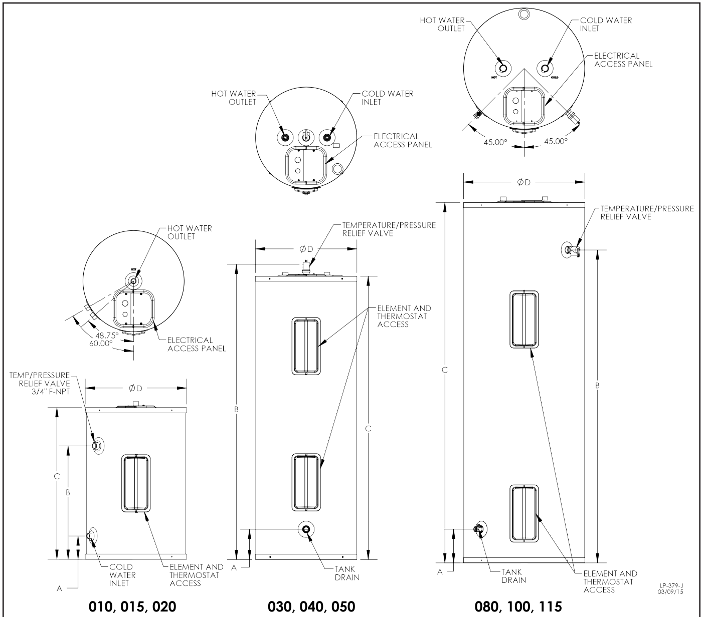
Figure 2 - Dimensional Drawing
